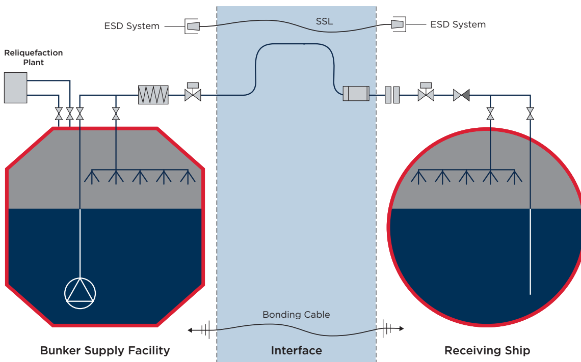
Figure 4.2: Typical detail of ammonia bunkering – FR to SR to P application.
