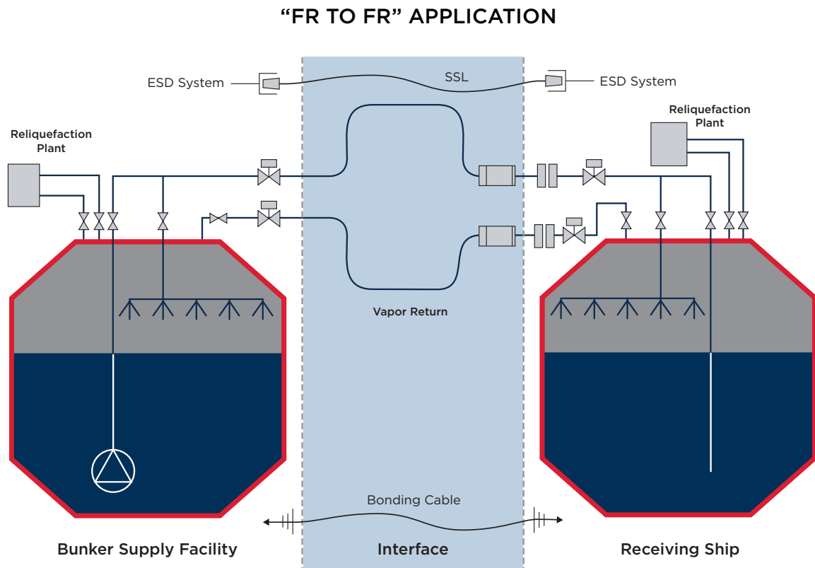
Figure 4.3: Typical detail of ammonia bunkering – FR to FR application.
