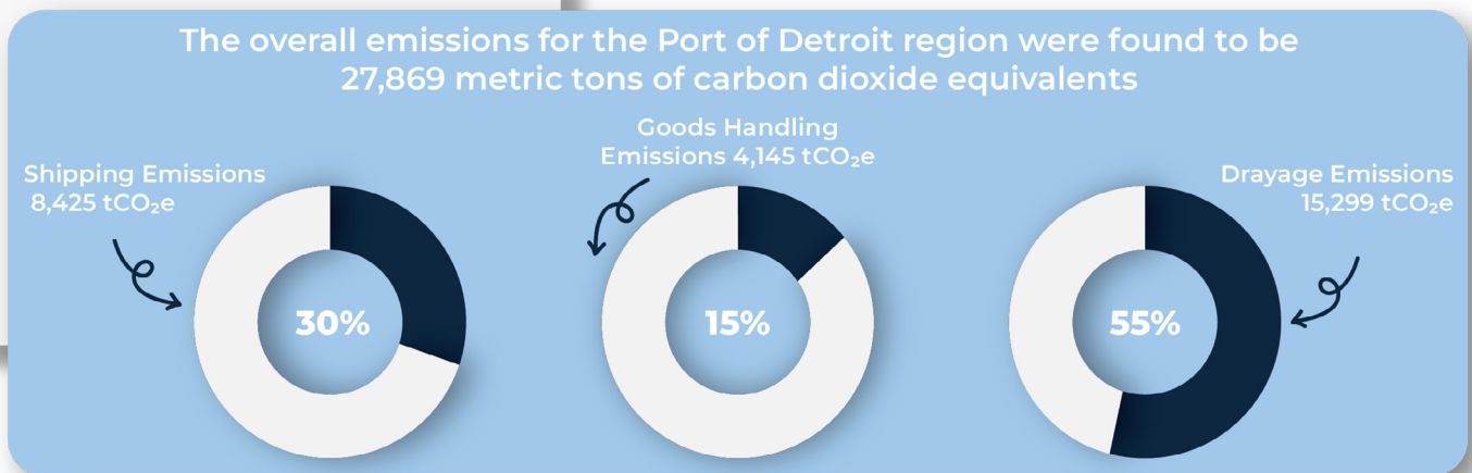
Figure 1: Overview of shipping, goods handling, and drayage emissions for the Port of Detroit.
