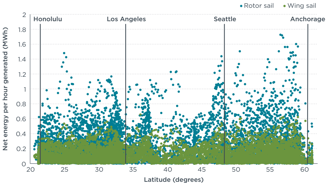
Figure 3. Wind-assisted propulsion net energy produced in one operating hour at different latitudes
