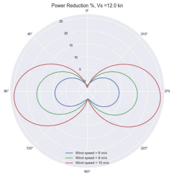
Figure 26. Main engine power reduction. Homocentric circles correspond to constant values of available power reduction.
