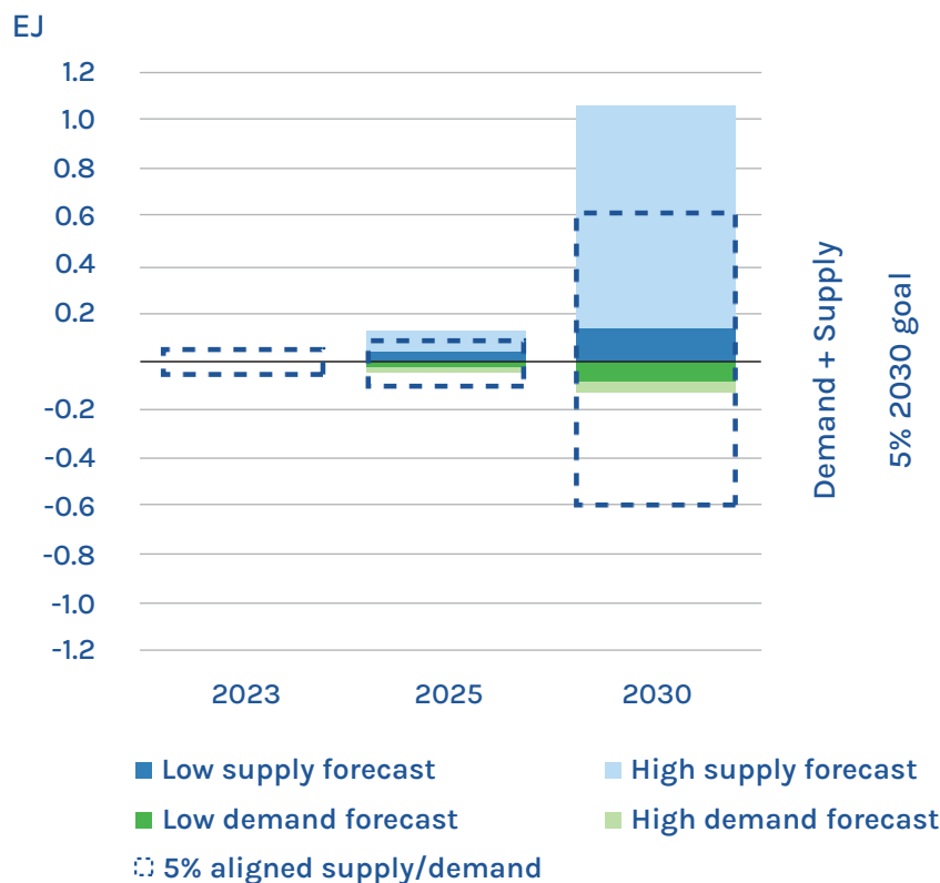
Figure 2. Estimated total SZEf supply and demand for shipping compared to 5% 2030 SZEf goal aligned supply/demand up to 2030 (i.e., 0.6 EJ in 2030). 14
