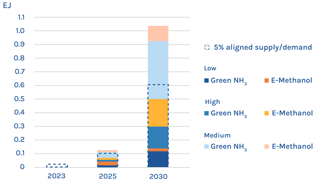
Figure 4. Estimated total supply from SZEf for maritime usage compared to 0.6 EJ 2030 requirement in line with the 5% SZEf 2030 goal. 21
