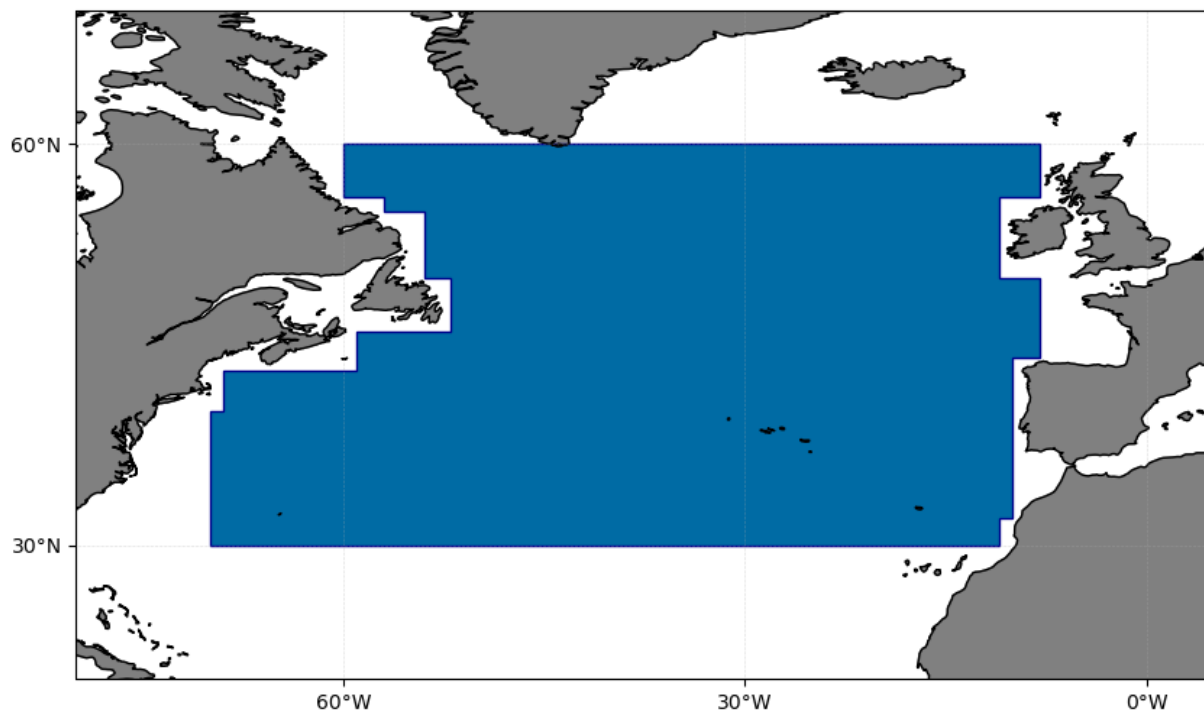
Figure 1: Definition of the extent of the North Atlantic
