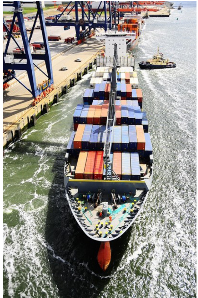
Figure 12: Berthing with ship astern
