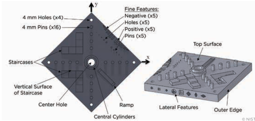
Figure 19 – NIST test artifact for PBF (Left: top view; right: oblique view)
