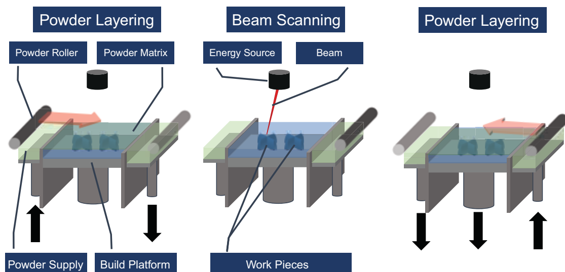
Figure 3 - Typical powder bed fusion build steps
