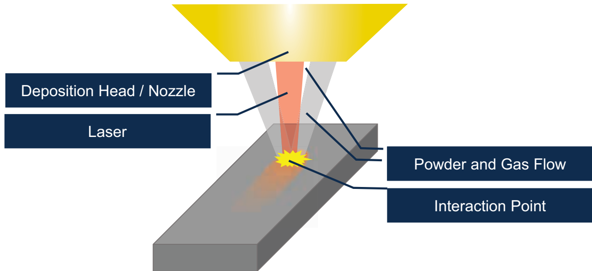
Figure 6 - Laser blown powder DED
