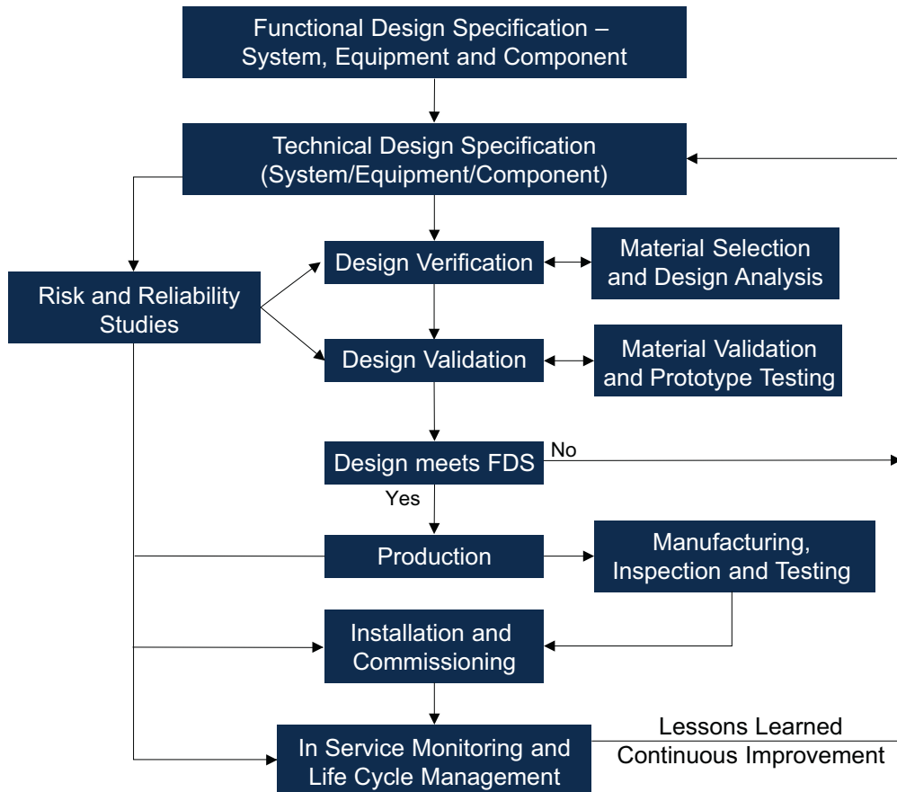
Figure 14 - General design process
