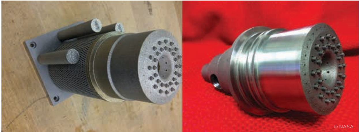
Figure 4 - NASA rocket injector, manufactured with PBF AM, reducing 115 parts to two
