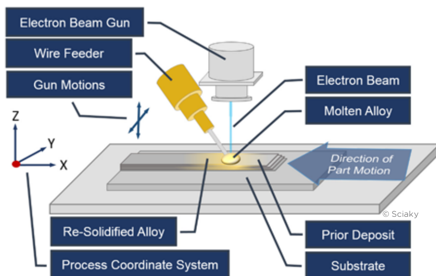
Figure 5 - Electron beam DED Illustration
