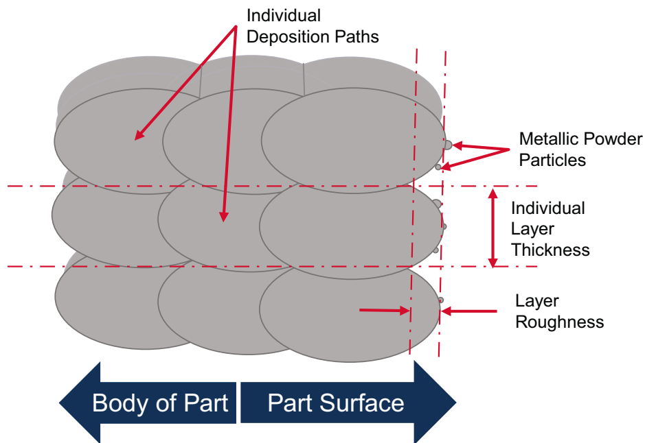
Figure 11 – Cross-section profile of a metal AM part, demonstrating surface roughness from two sources: Layer roughness and from metallic particles adhered to the surface
