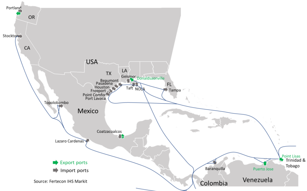
Figure 15. Ammonia terminals in the Caribbean Basin and North America (not showing the US east coast). Source Fertecon IHS Markit.
