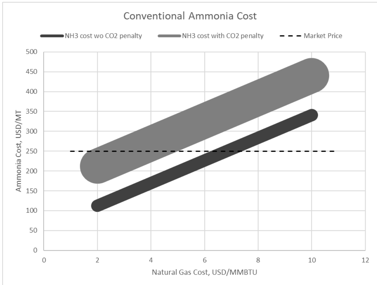
Figure 5. Estimated production cost and market price of conventional ammonia (definition see text).
